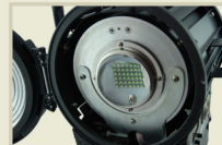
D-LFS series 3 layers of aspheric lens optical system
