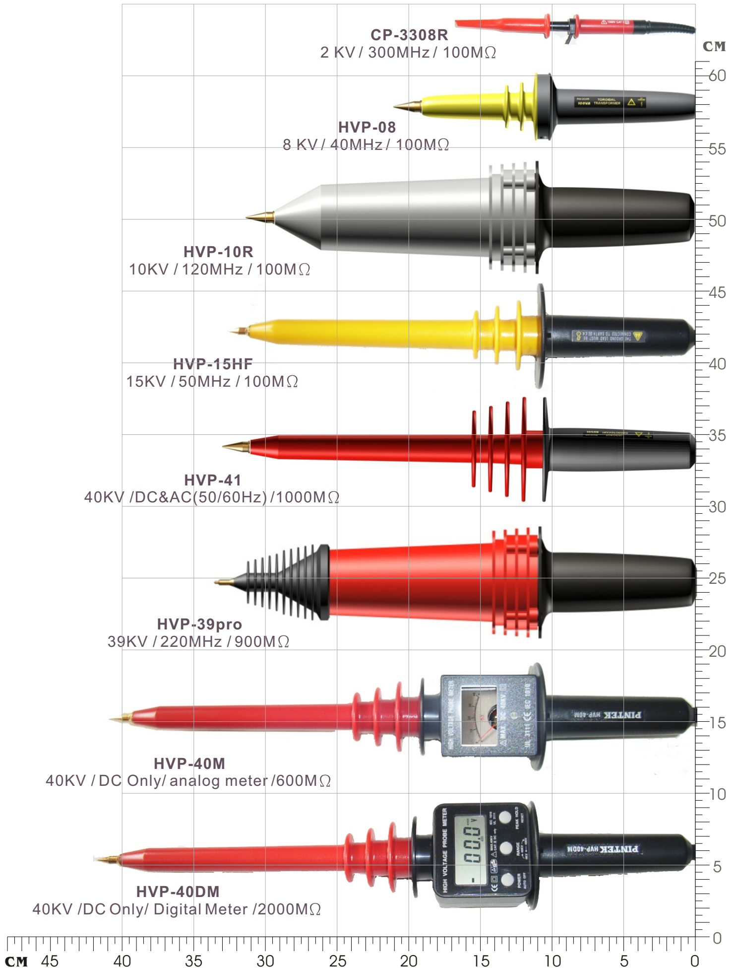
High Voltage Probe Dimension Comparison Fig.
